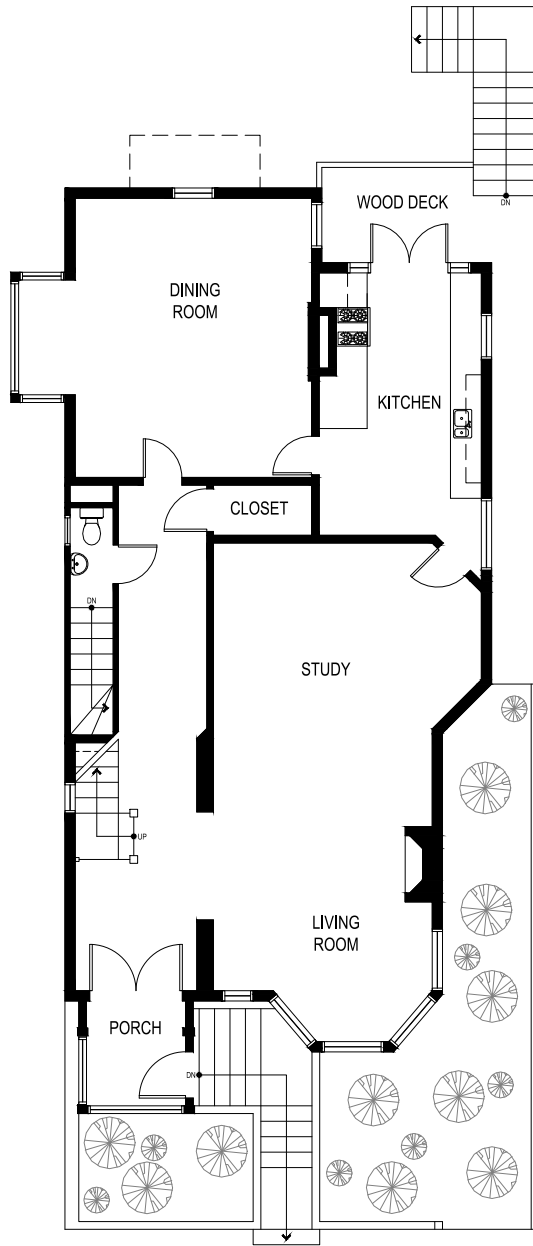
FIRST FLOOR
